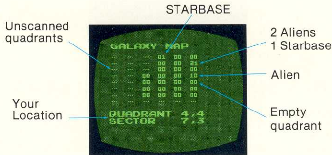
Figure 2. GALAXY MAP
